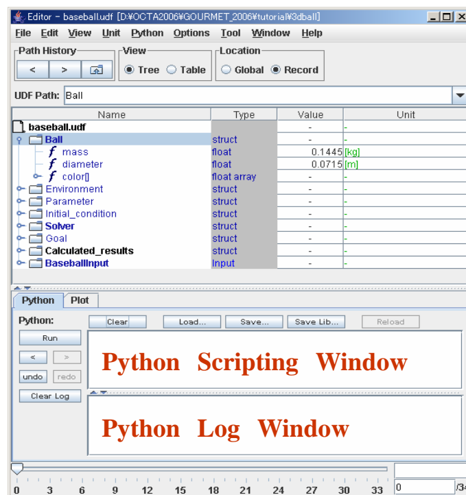
Figure 2: Tree View of Editor
