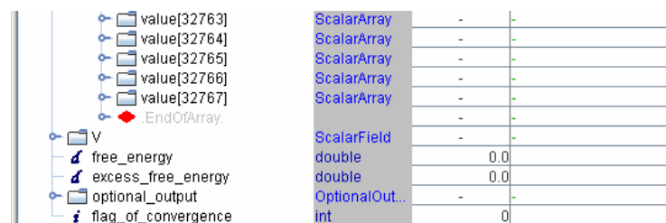
Figure 13: "EndOfArray"
